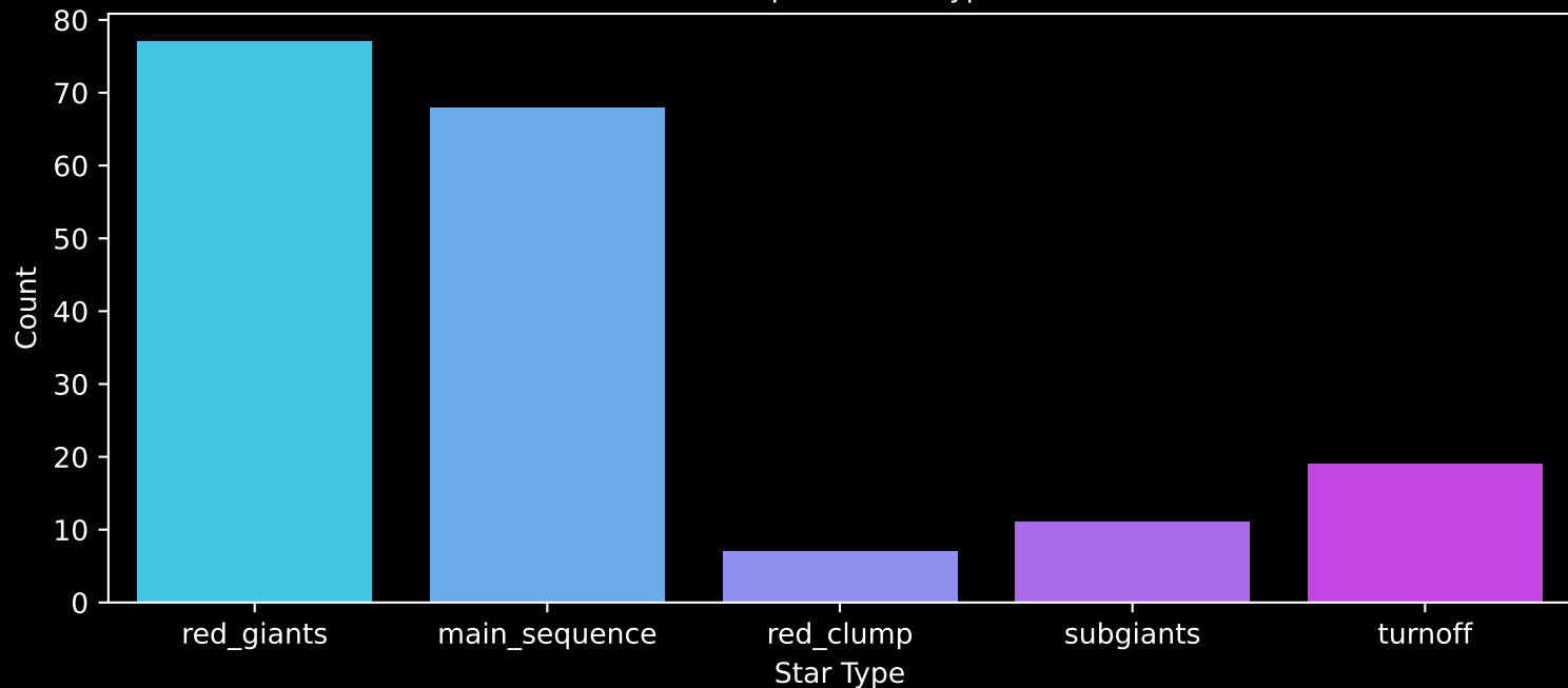
APOGEE DR17 Field: [TRIAND-4] Count plot of Star Type
