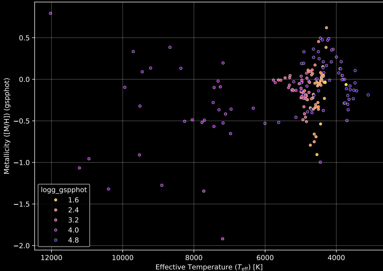
APOGEE DR17 Field: [TRIAND-4] Stellar Population Parameters (n= 182)
