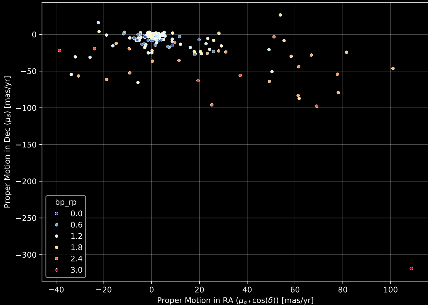
APOGEE DR17 Field: [TRIAND-4] Proper Motion Diagram (n= 182)
