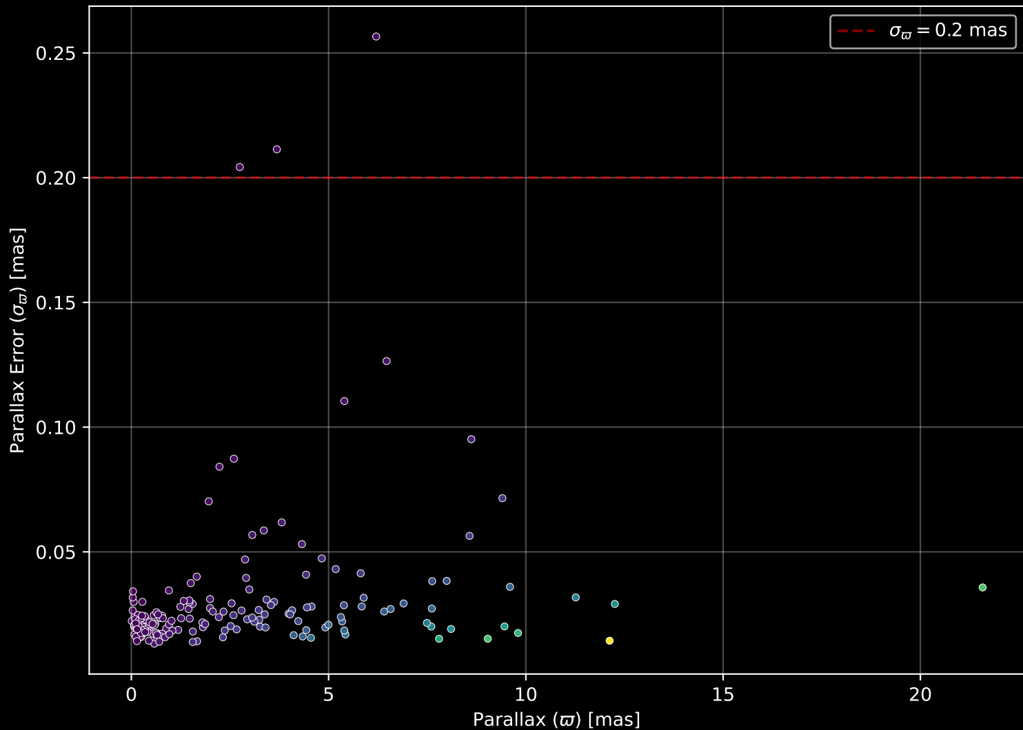
APOGEE DR17 Field: [TRIAND-4] Parallax Quality (n= 182)
