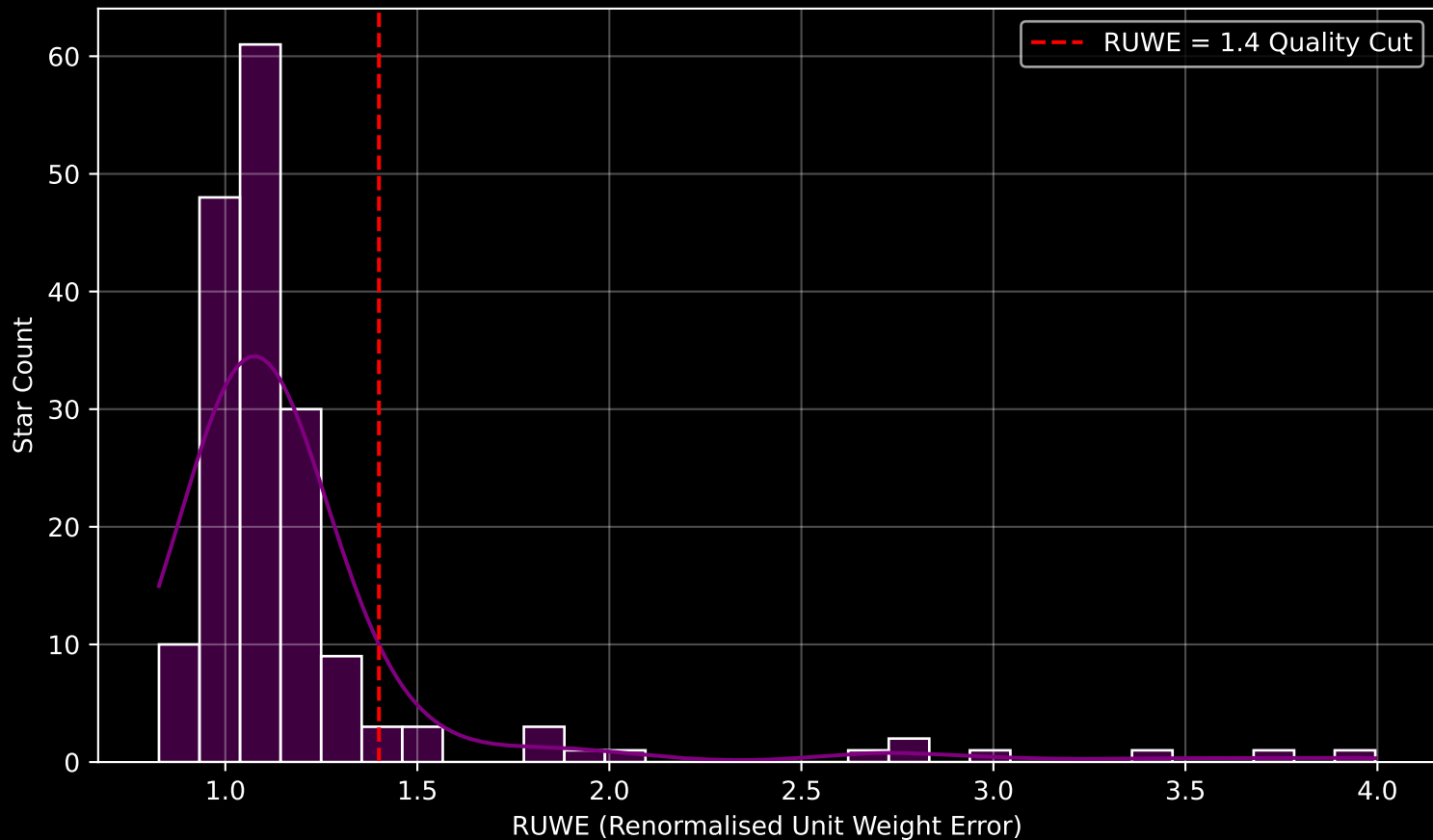
GAPOGEE DR17 Field [TRIAND-4] RUWE Distribution (n= 176)
