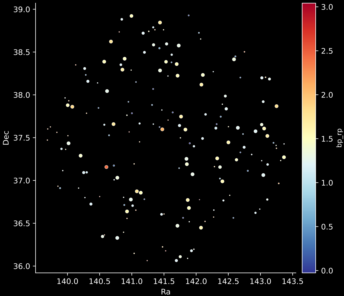
APOGEE DR17 Field: [TRIAND-4] Stars: 182
