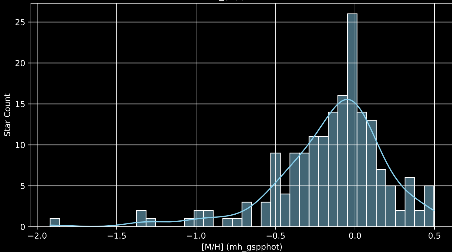
APOGEE DR17 Field: [TRIAND-4 [M/H] (mh_gspphot) (n= 180)
